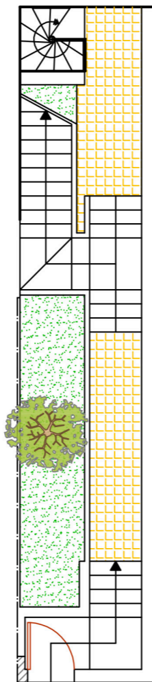
PIANO TERRA Scala 1:100
