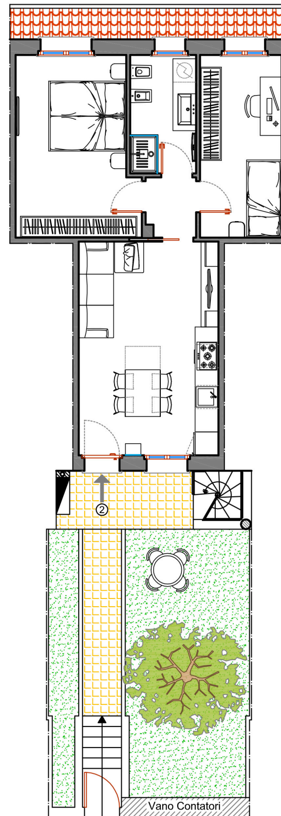
PIANO TERRA Scala 1:100
